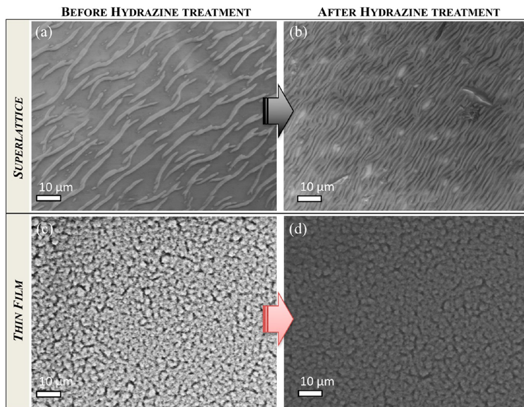
Figure 6. Preparation and characterization of PbS SL membranes and PbS spin-cast solids on SiO 2 /Si wafer ( \sim 1 \text{ cm} \times 1 \text{ cm} ). SEM images of (a, b) SL membranes and (c, d) spin-cast solids of PbS NCs transferred on top of SiO 2 /Si wafer substrates (a, c) before and (b, d) after 1 M hydrazine treatment for 4 h, so as to investigate the influence of the ligand exchange treatment on the uniformity and homogeneity of the final NC solids.
